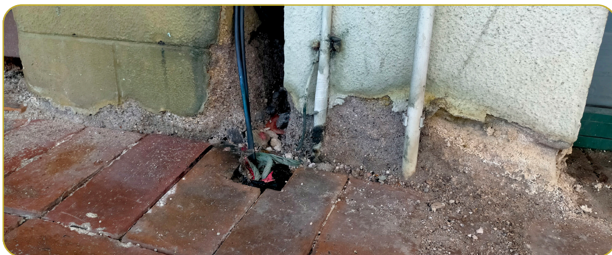
Figure 23 Deterioration of building materials at ground level (photo: Kim Smith, January 2024).
