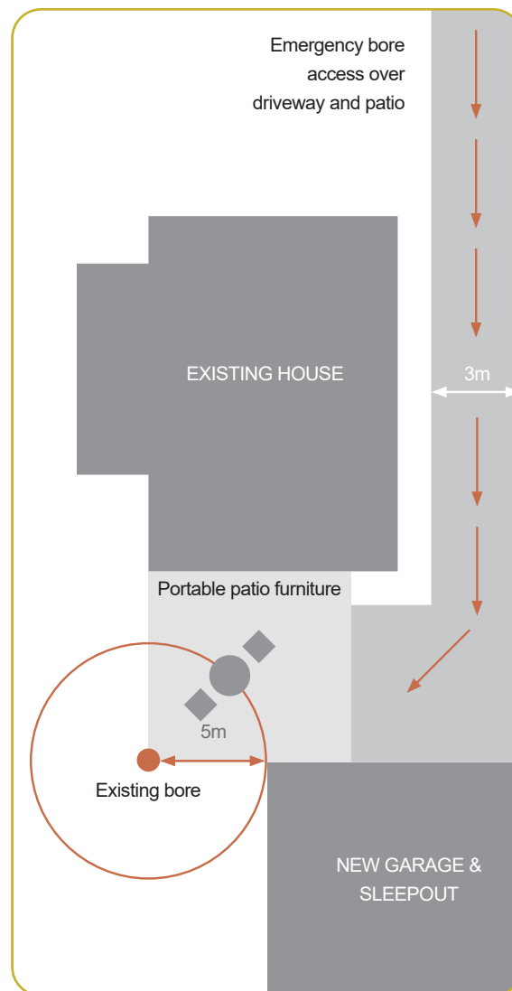
Figure 19 Conceptual example of site layout to maintain access to an existing bore with development of new garage and sleepout.
