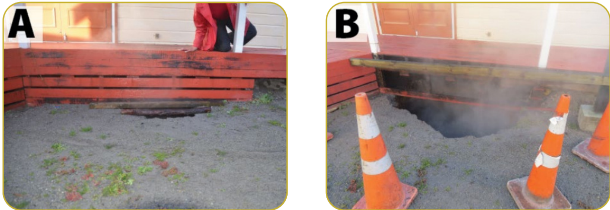
Figure 9 A collapse hole developing at Whakarewarewa Village over eight days in September 2012. Roof-fed stormwater disposal to shallow depth drove the creation of the feature (these images were originally published in Fitzgerald, 2022)
