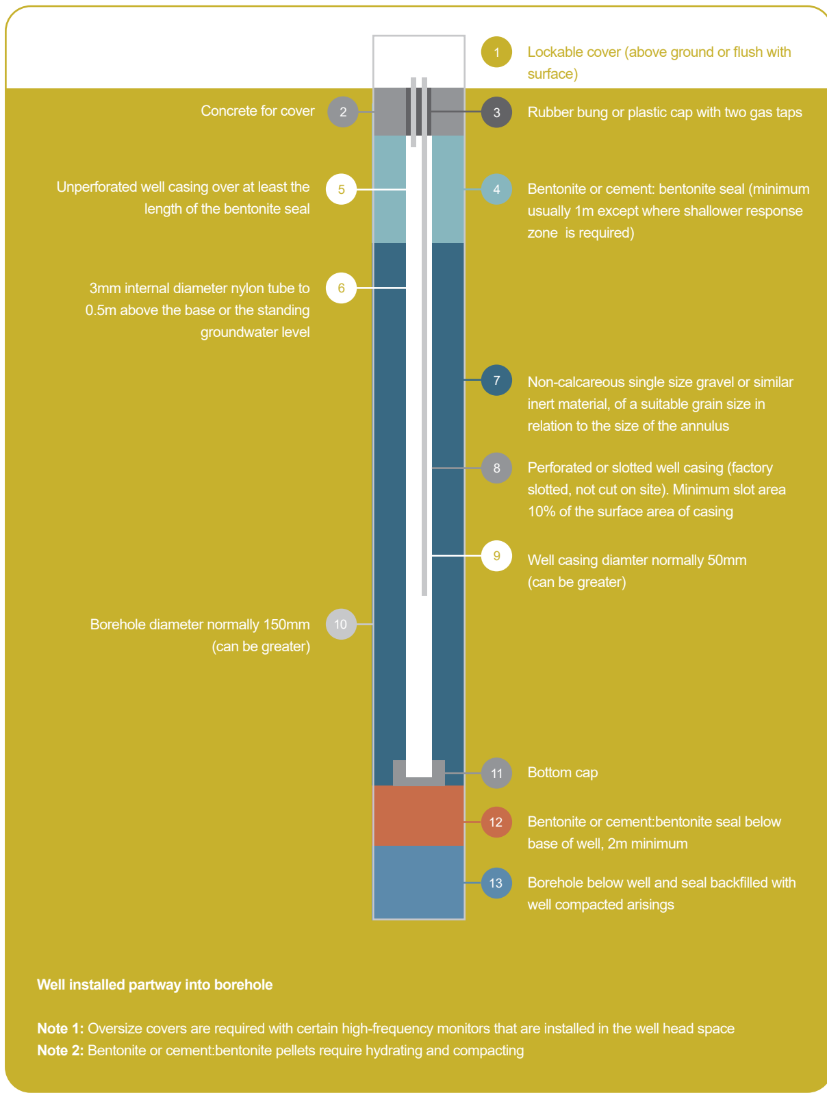
Figure 18 Typical well design (Based on the diagram in BS 8576:2013).
